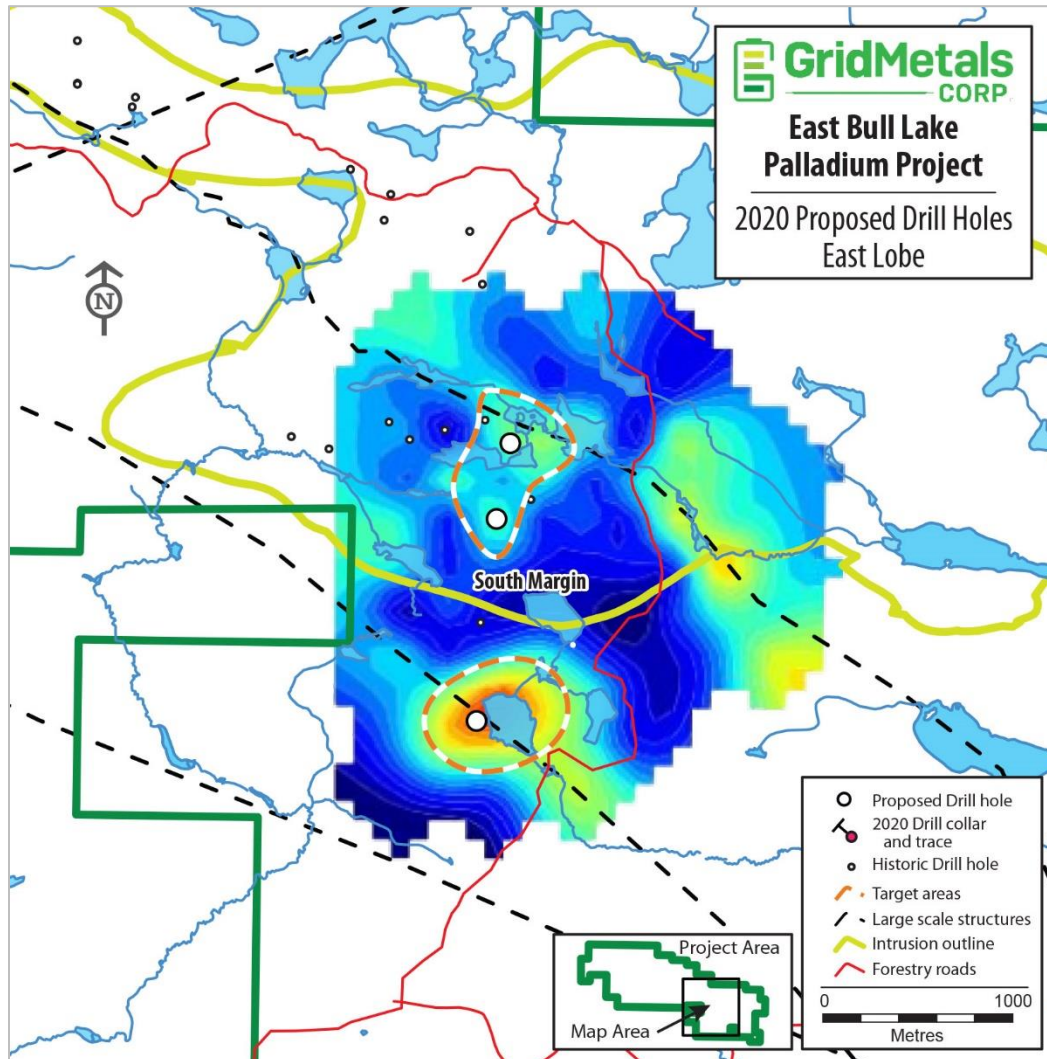
Figure 3. Location of proposed drill hole collars that are under consideration for the next phase of drilling on the South Margin target area in the East Lobe of the EBL intrusion. Background map is a colour gradient image of the near surface apparent resistivity from the 2020 MT survey.
