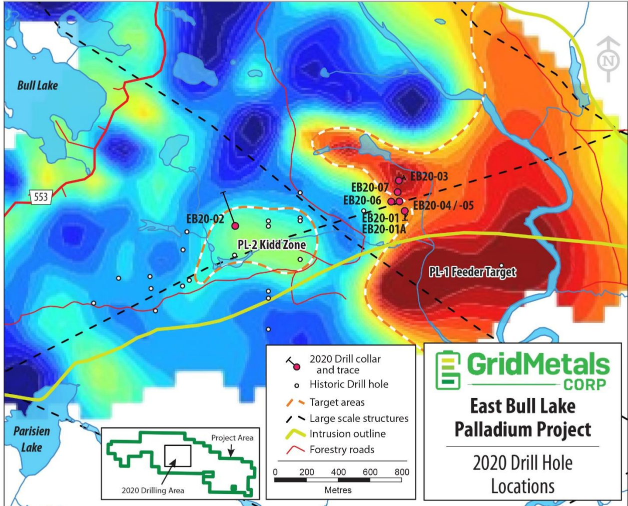
Figure 1. Location of completed 2020 drill holes in the Parisien Lake area, western lobe, EBL intrusion. Drill target areas and associated near surface geophysical anomalies (PL-1, PL-2) also shown. Background image is a colour gradient map of near surface apparent resistivity based on the 2020 MT survey on which warmer colours have lower resistivity.
